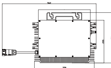
130/160/180/200/220 G4 (4MPPT) Mounting
